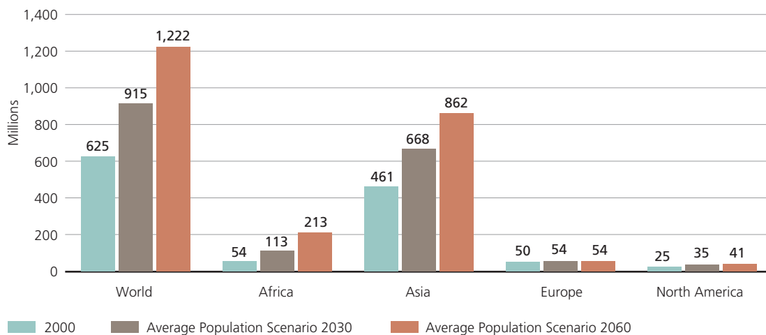
Figure 4: Population living in low-lying coastal areas
